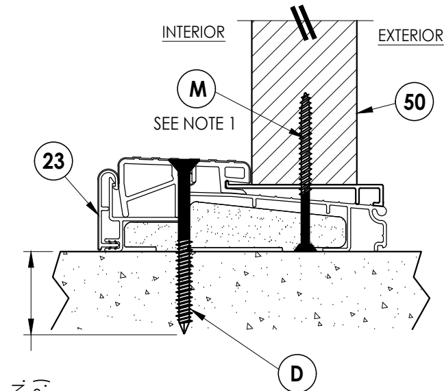
7 5 VERTICAL CROSS SECTION Inswing sill
