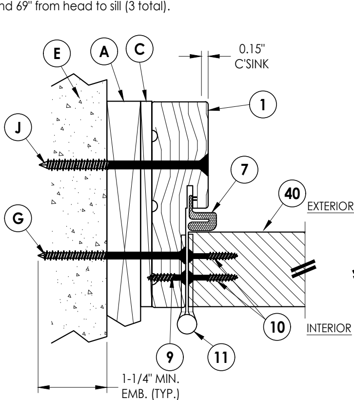
3 6 HORIZONTAL CROSS SECTION Inswing shown (Outswing similar) 1X Buck Construction
