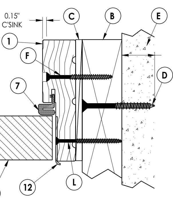
2 6 HORIZONTAL CROSS SECTION Inswing shown (Outswing similar) 2X Buck Construction
