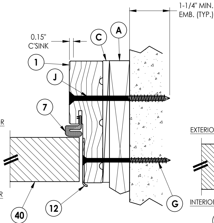
4 6 HORIZONTAL CROSS SECTION Inswing shown (Outswing similar) 1X Buck Construction
