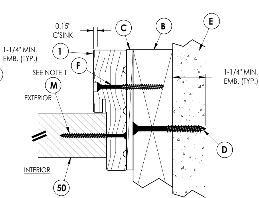
5 6 HORIZONTAL CROSS SECTION Inswing shown (Outswing similar) 2X Buck Construction
