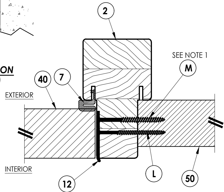
7 6 HORIZONTAL CROSS SECTION Inswing shown (Outswing similar)
