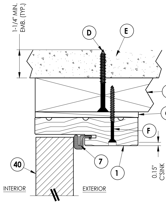
1 5 VERTICAL CROSS SECTION Inswing shown (Outswing similar) 2X Buck Construction
