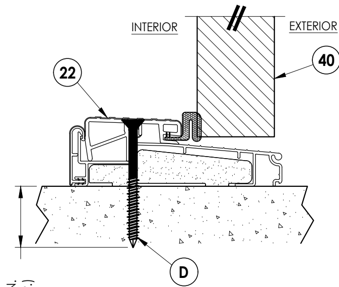
5 5 VERTICAL CROSS SECTION Outswing sill
