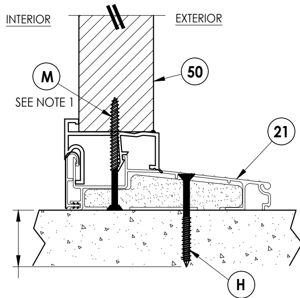
6 5 VERTICAL CROSS SECTION Inswing sill
