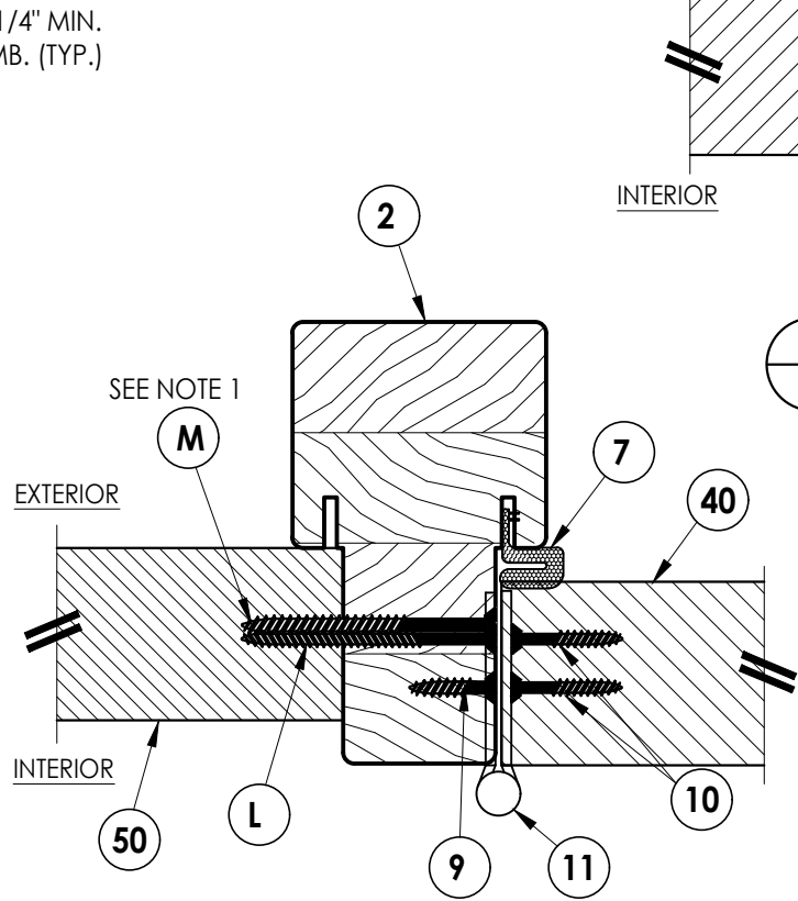
6 6 HORIZONTAL CROSS SECTION Inswing shown (Outswing similar)
